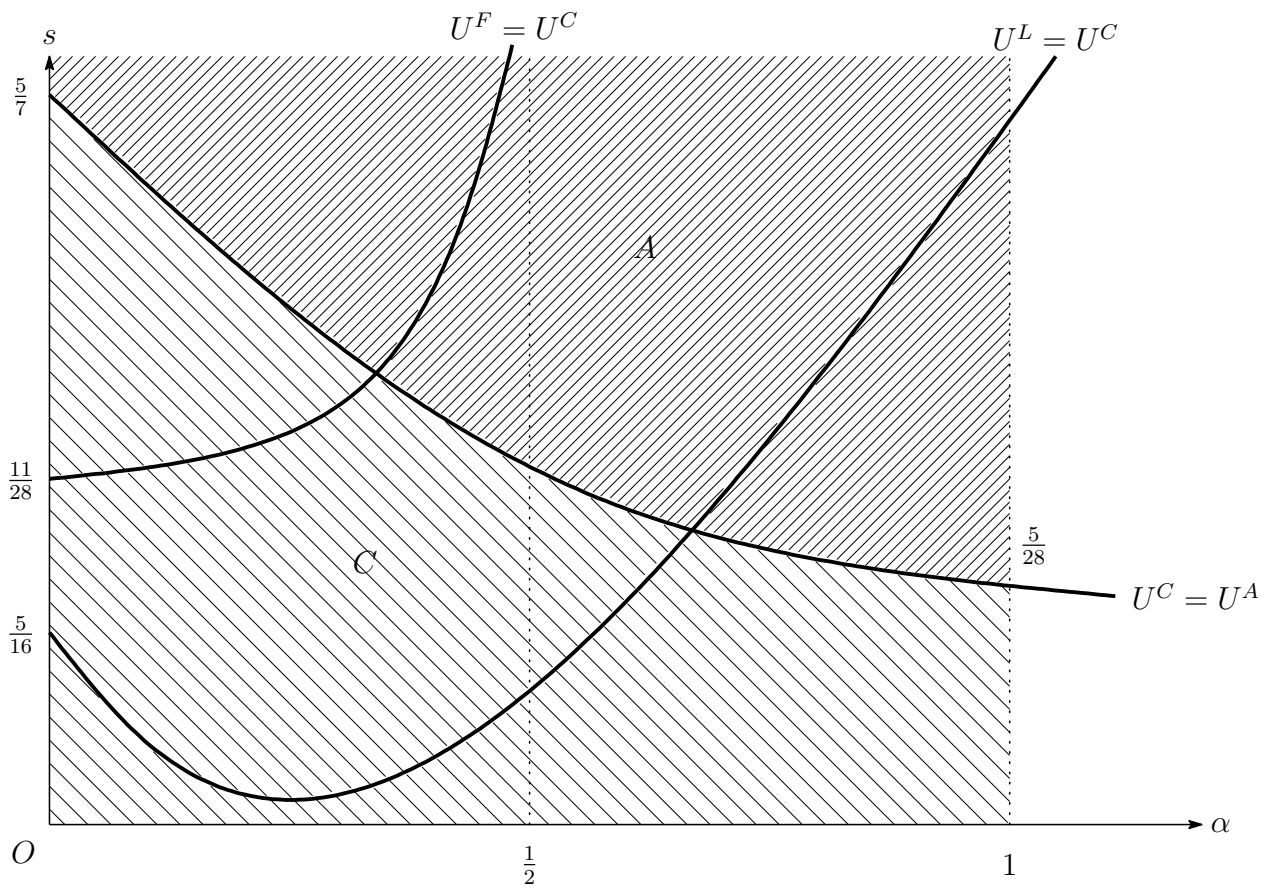
Figure 2: Regions for Cournot-Nash and autarkic outcomes in the symmetric case
