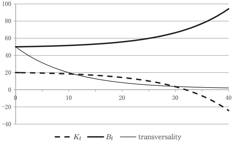
Figure 2. A Numerical Example
